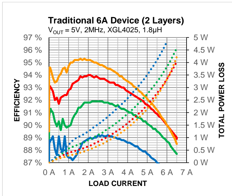
Figure 7: Traditional 6A Device Efficiency and Total Power Loss on a 2-Layer PCB
