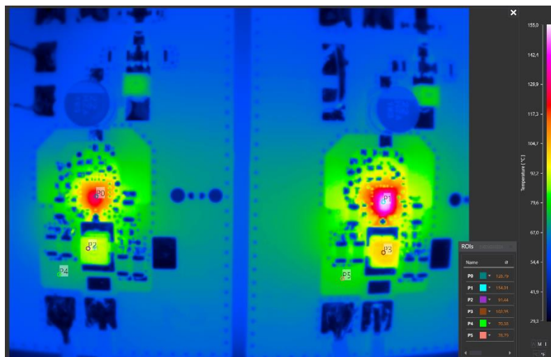
Figure 11: T_{PACKAGE} vs. I_{LOAD} of MPQ4326-AEC1 and Traditional 6A Device
