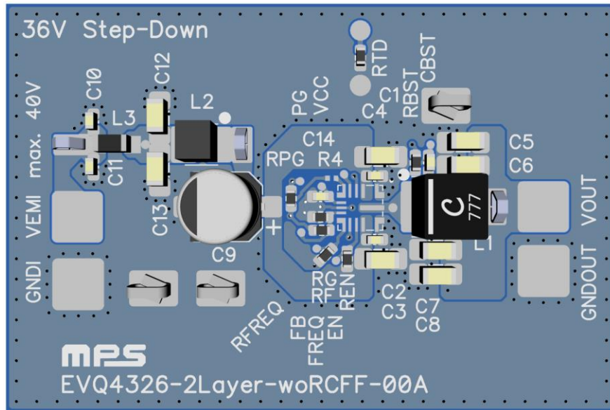
Figure 2: MPQ4326-AEC1 2-Layer PCB (60mmx40mm) Component Placement
