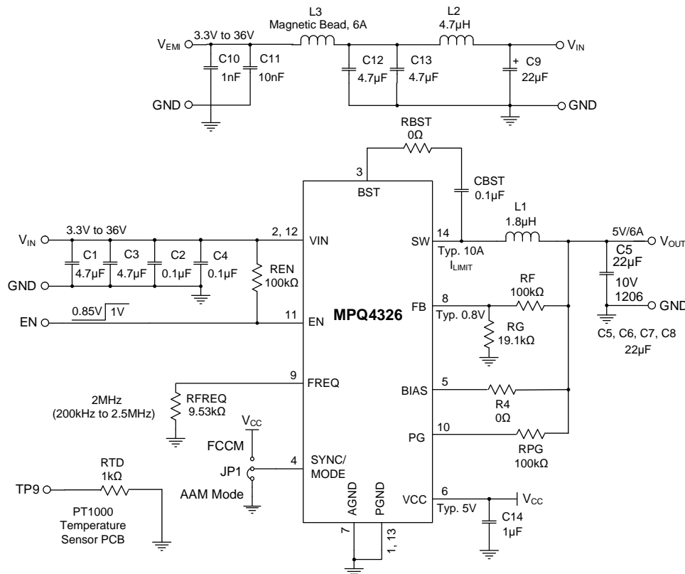
Figure 1: MPQ4326-AEC1 Typical Application Schematic
