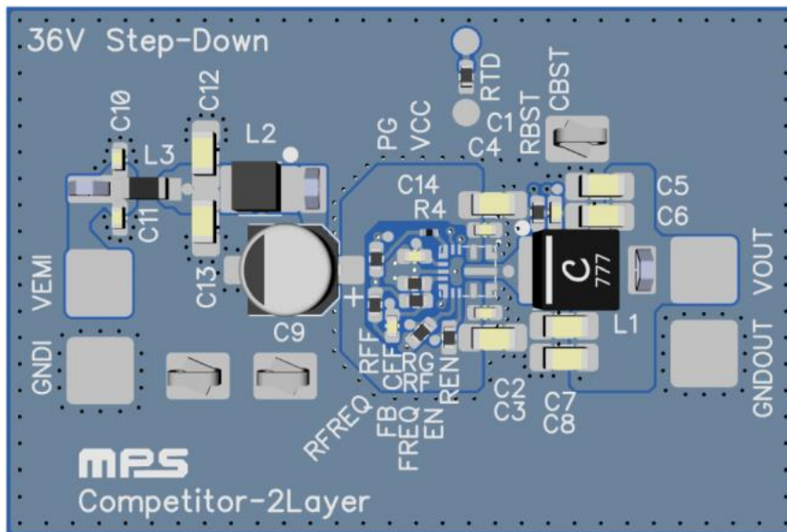
Figure 3: Traditional 6A Device 2-Layer PCB (60mmx40mm) Component Placement
