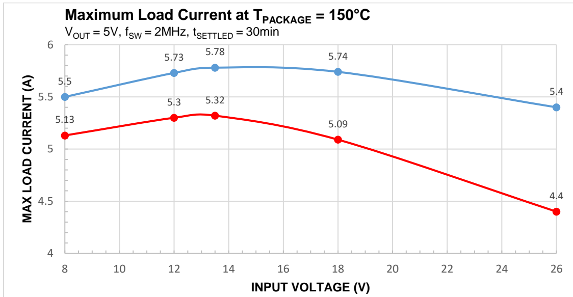
Figure 8: Maximum Load Current at T_{PACKAGE} = 150^{\circ}C
