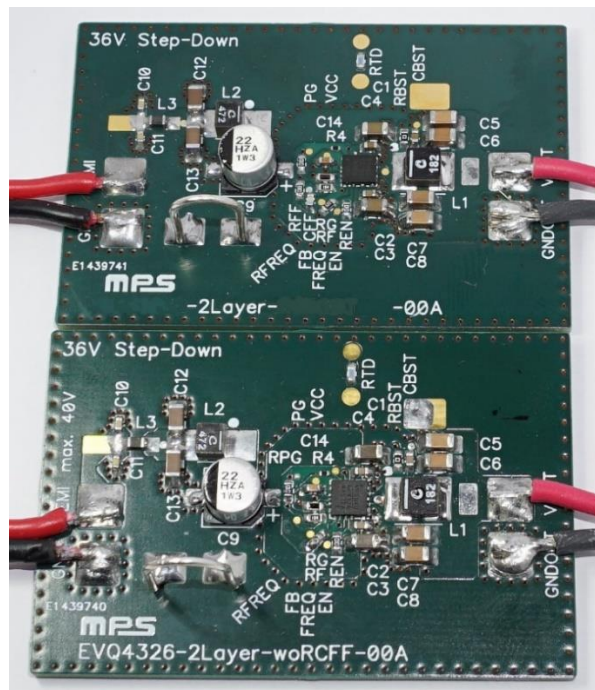
Figure 4: Comparison of 2-Layer PCBs for the MPQ4326-AEC1 and a Traditional 6A Device
