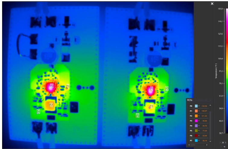
Figure 10: MPQ4326-AEC1 vs. Traditional 6A Device at T_{PACKAGE} = 150^{\circ}C and Different I_{LOAD\_MAX} Values
