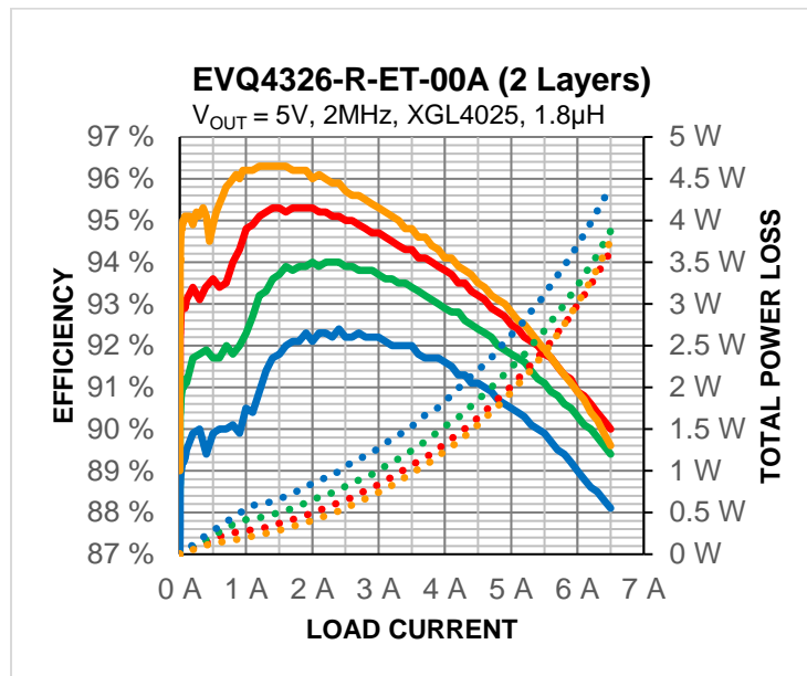
Figure 6: MPQ4326-AEC1 Efficiency and Total Power Loss on a 2-Layer PCB
