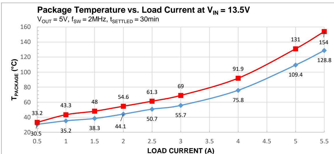
Figure 9: Package Temperature vs. Load Current at V_{IN} = 13.5V
