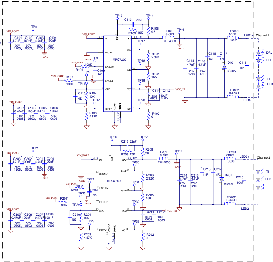
MPO7200 2 Channel buck-boost, channel1 for DRL&PL LED, channel2 for TI LED
