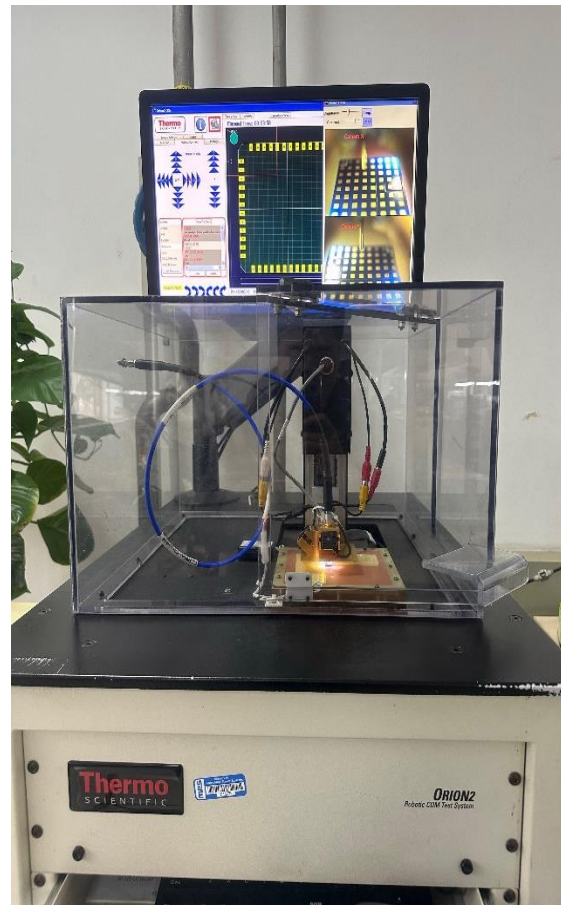
CDM ESD Machine
