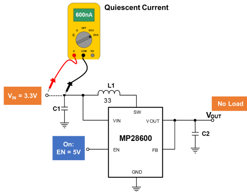
Figure 4: Measuring I_Q
