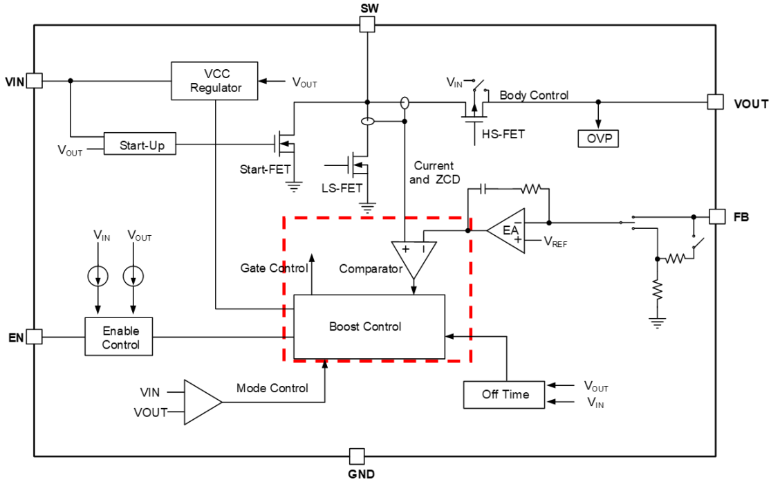
Figure 5: I_q in an IC Circuit
